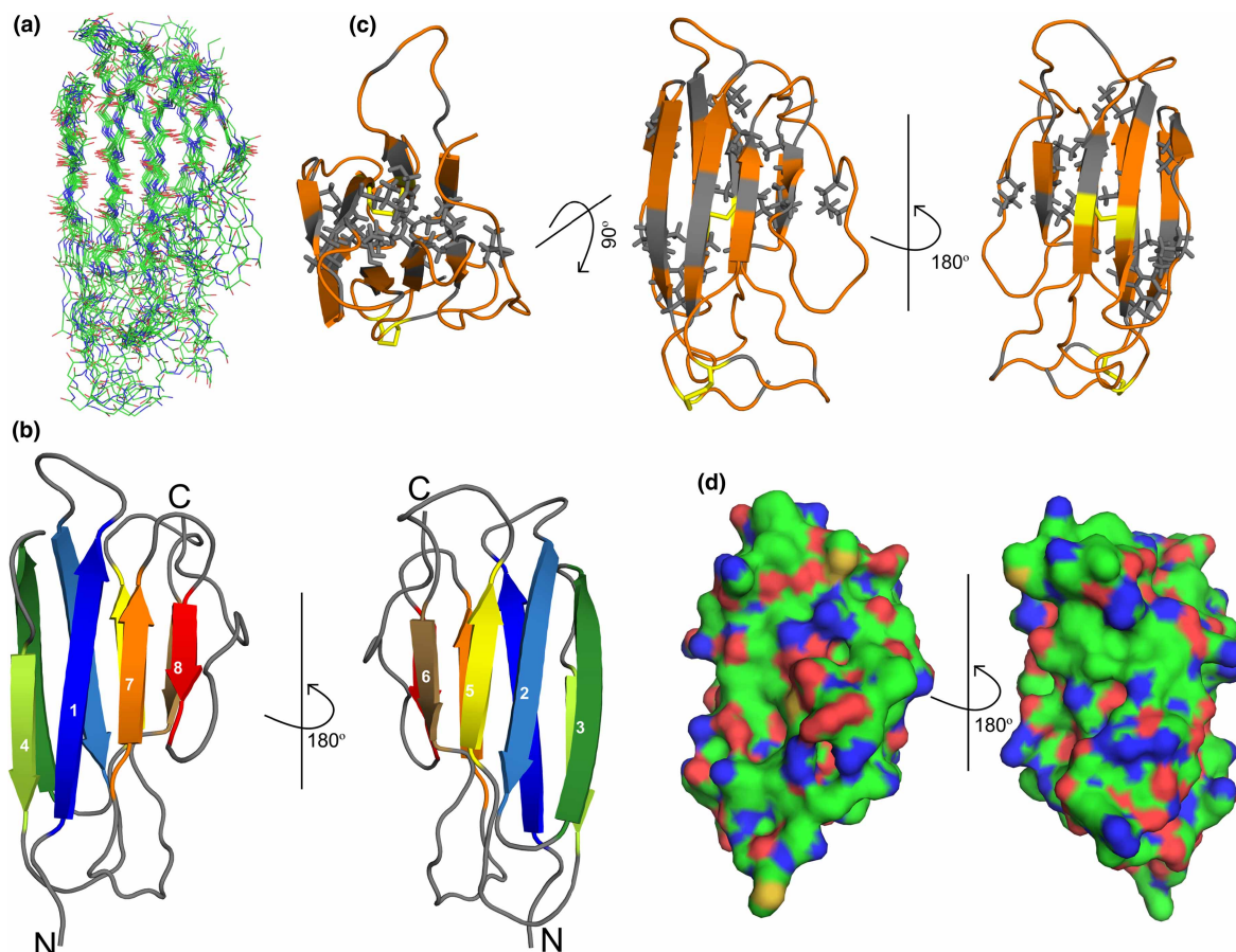
Figure 4. 3D structure of SPH15.
