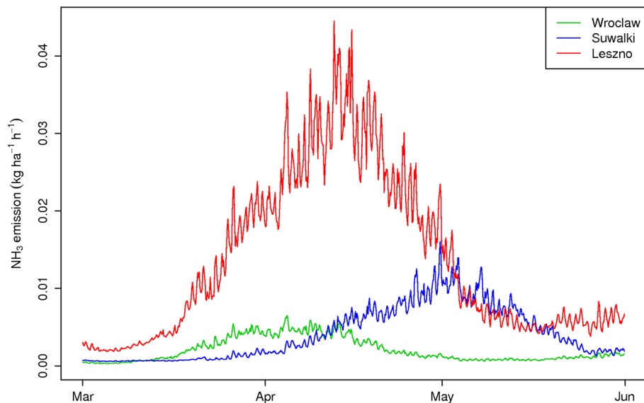
Figure 5. The hourly variation in simulated NH 3 emissions for POLREGUL scenario. Data from March to May for three locations in Poland (Wrocław, Suwałki and Leszno).
