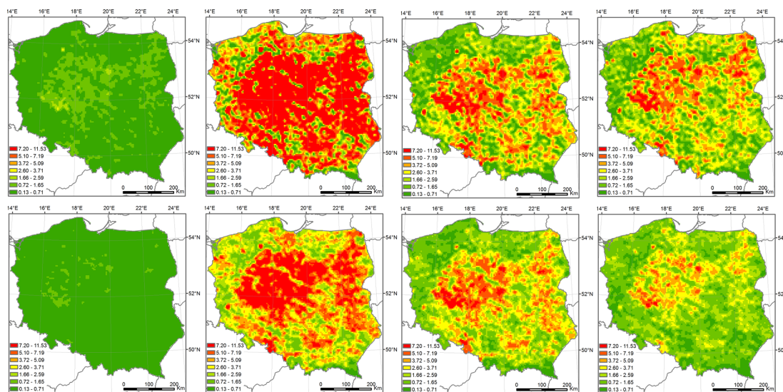
Figure 4. Top: spatial distribution of \text{NH}_3 emissions over Poland for 15 February, 15 April, 15 June and 15 September 2010 at 12:00–15:00 UTC [ \text{g ha}^{-1} 3 \text{ h}^{-1} ]. Bottom: monthly mean ammonia concentrations calculated with the FRAME model (POLREGUL) for February, April, June and September 2010.
