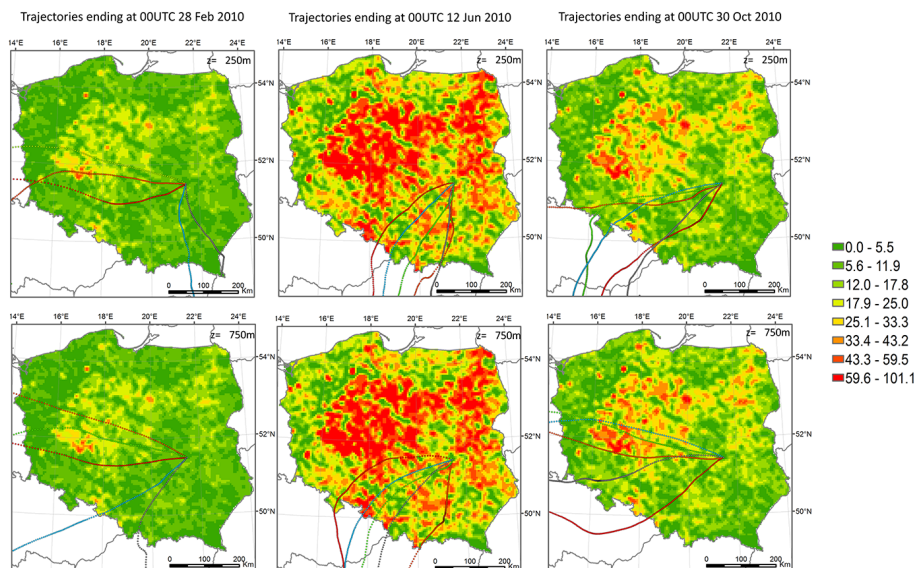
Figure 8. Thirty-six-hour backward trajectories ending in Jarczew during episodes (25–27 February 2010, 09–11 June 2010, 10–29 October 2010) with high \text{NH}_3 measured concentrations. The first trajectory (grey) starts at 12:00 of the first day of each episode, and then starts every 6 h, and are presented in the following colours: blue, green, orange and red. Spatial distribution of modelled ammonia emission during the episodes (unit: \text{g ha}^{-1} 48 \text{ h}^{-1} ).
