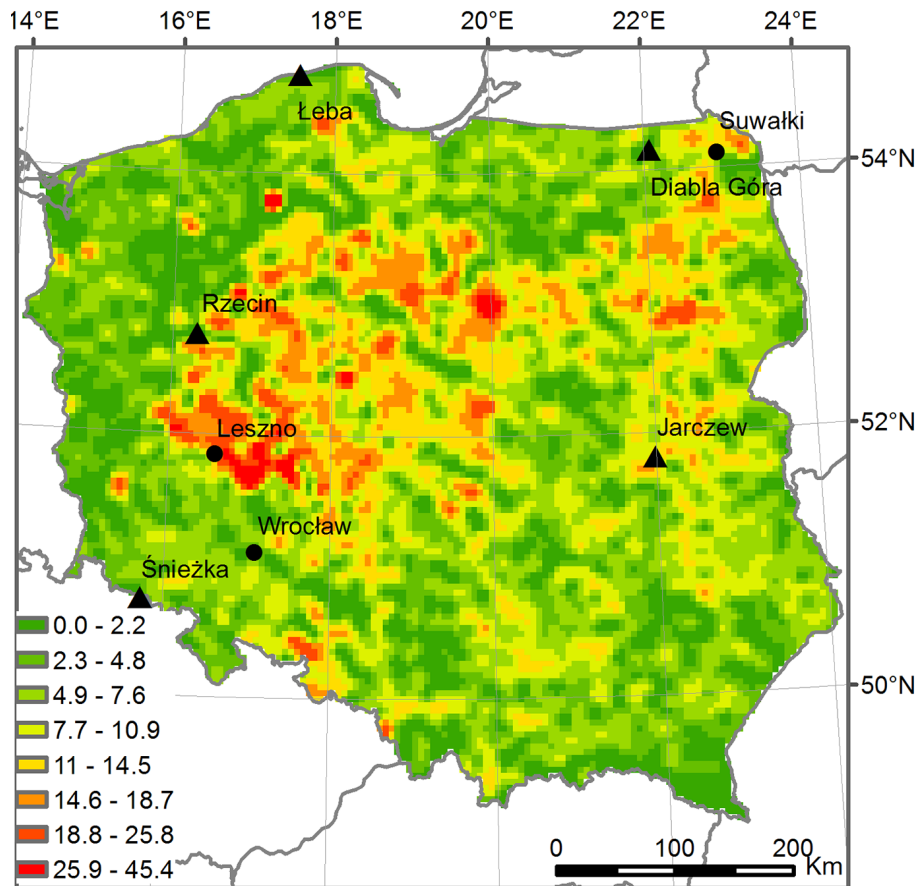
Figure 1. Total annual emission of \text{NH}_3 in 2010 [ \text{kg ha}^{-1} \text{ year}^{-1} ]. \text{NH}_3 measurement sites indicated by triangles. Additional locations discussed in the paper indicated by circles (Wrocław, Leszno, Suwałki).
