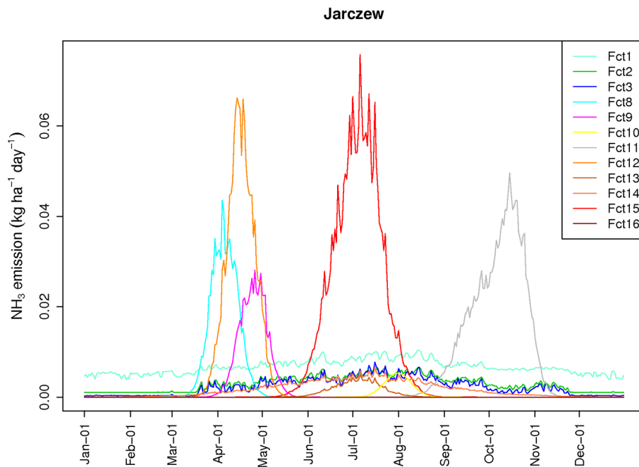
Figure 3. Time series of the seasonal variation in emission (POLREGUL run) for various agricultural emission categories in Jarczew (functions (Fct) described in Table 1).
