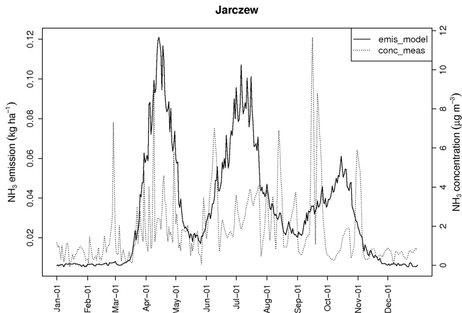
Figure 7. Modelled emission and measured concentration for the Jarczew station.
