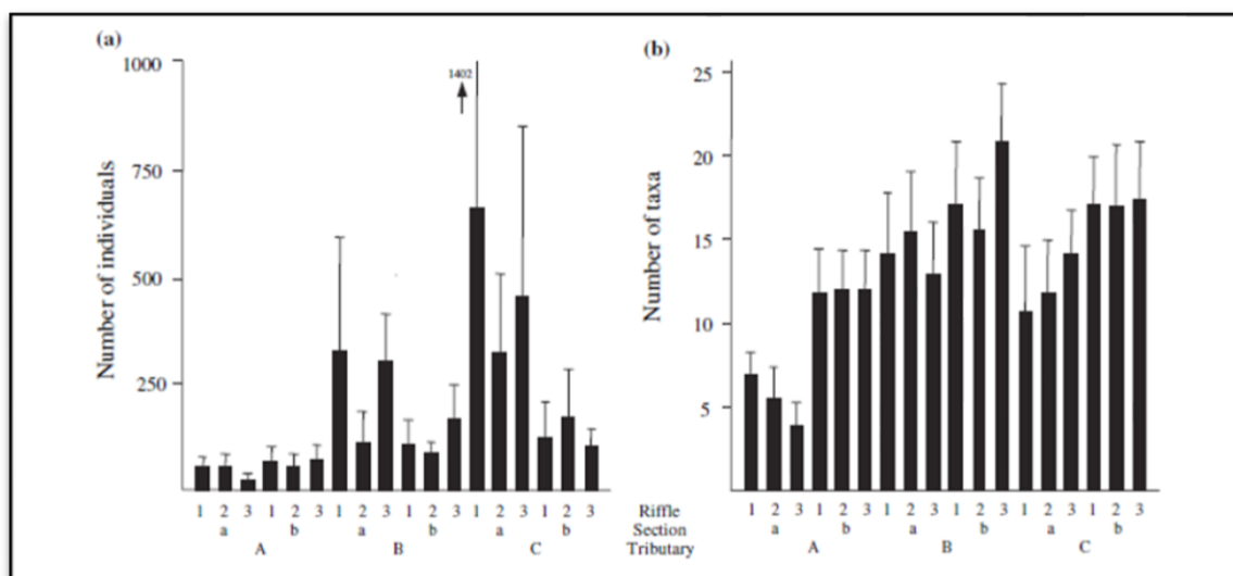
Figure 2:6 Mean ( \pm 1 SE) number of individuals and taxa per sample in each riffle. Capital letters (A, B, C) refer to different tributaries, small letters (a, b) to upstream versus downstream sections within each tributary, and numbers (1, 2, 3) to riffles within each section (Heino et al. , 2004, 1234).
