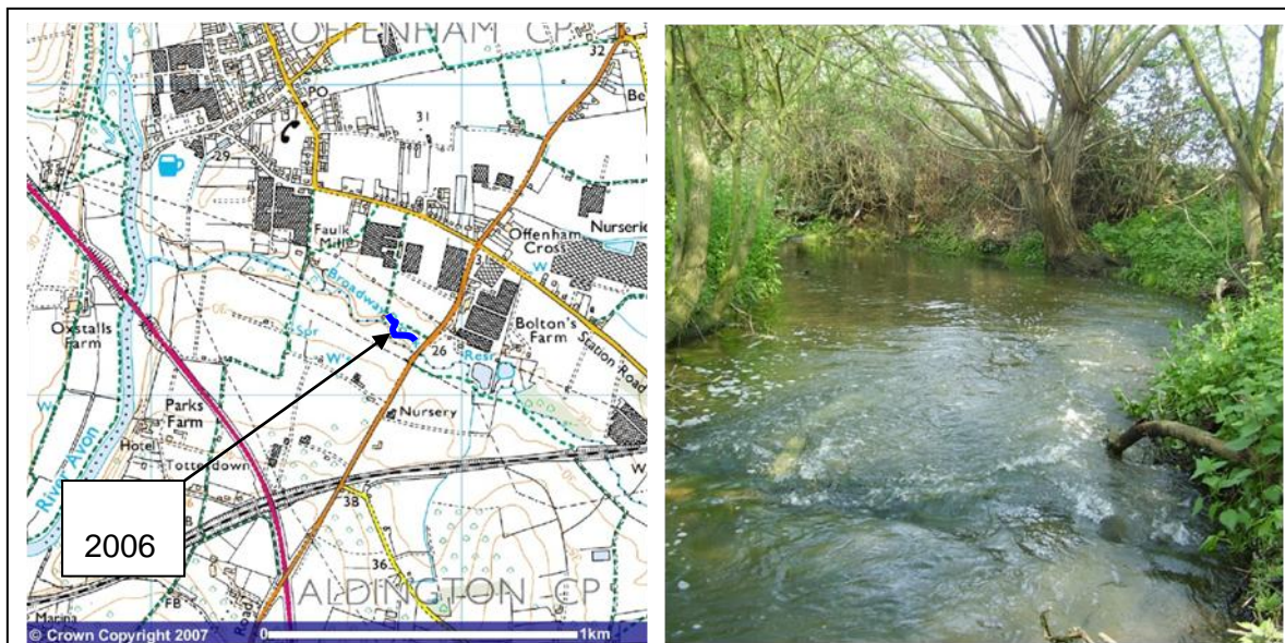
Figure 3:3 Location and typical view of Badsey Brook (marked Broadway Brook) near Offenham, Worcestershire. NGR SP 057 452 (Map source: www.ordnancesurvey.co.uk/oswebsite/getmap/ , 25/10/2007.)
