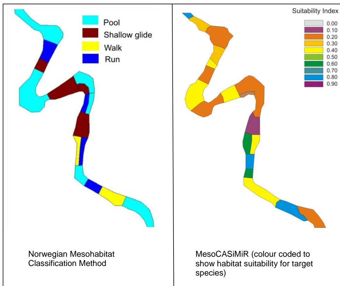
Figure 2:10 Examples of Norwegian Mesohabitat Classification Method and MesoCASiMiR showing lateral diversity allowed. From Maddock and Hill (2005).
