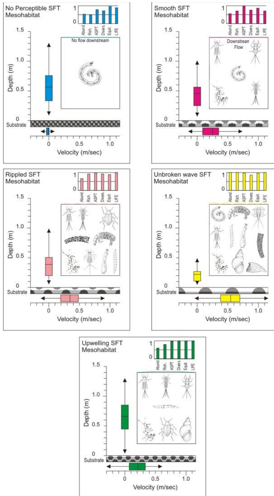
Figure 7:1 Summary diagram showing physical and biological features of Surface Flow Type mesohabitats from data gather in this research.
