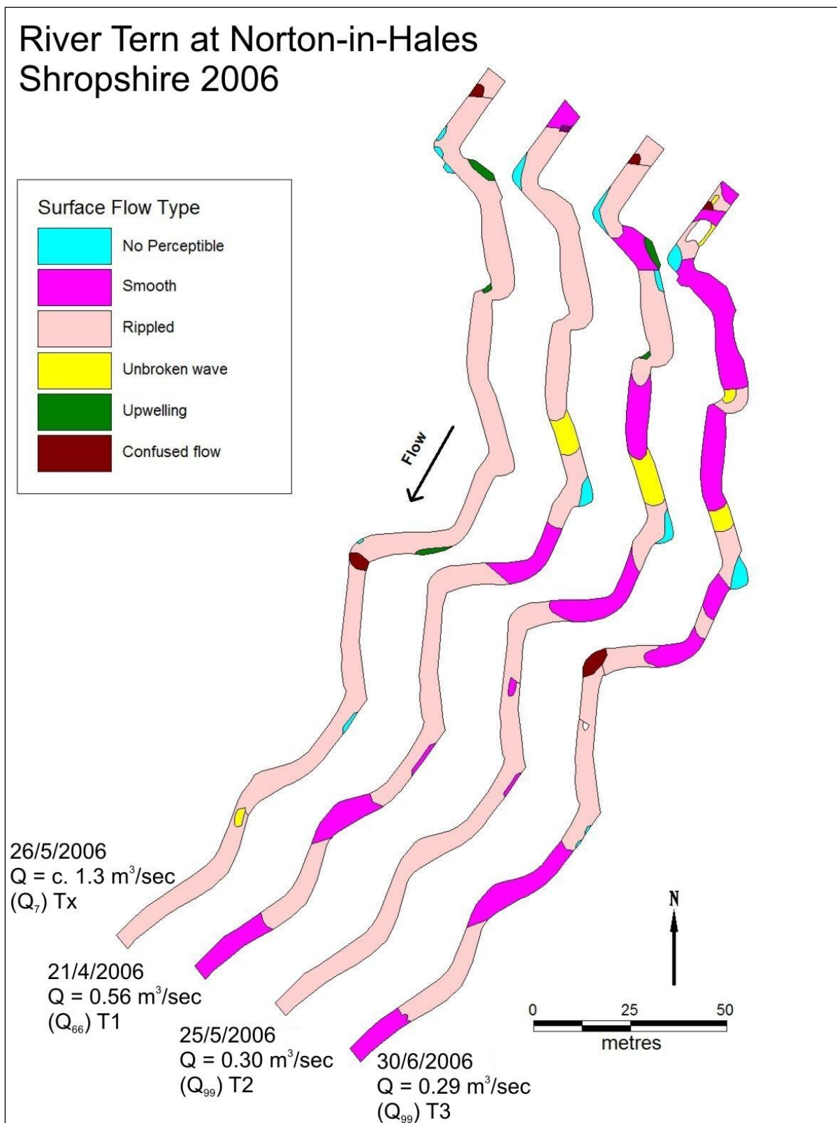
Figure 5:13 Surface Flow Type mesohabitats from four surveys of the same reach of River Tern, Shropshire during 2006. Key: T – River Tern, Q – Discharge.
