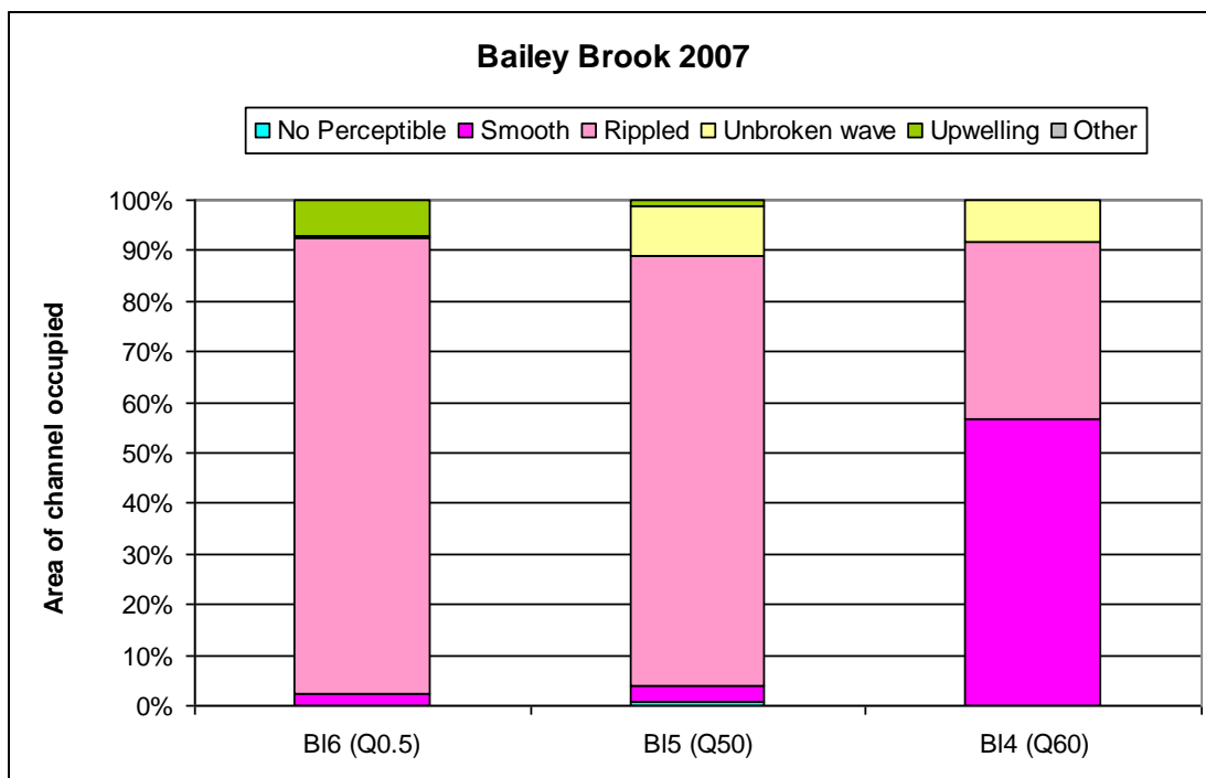
Figure 5:12 Relative proportions of the channel occupied by Surface Flow Type mesohabitats in Bailey Brook, Shropshire during three surveys during 2007, data derived from SFT maps drawn by eye onto channel plan. Key: BI - Bailey Brook, Q – Discharge.
