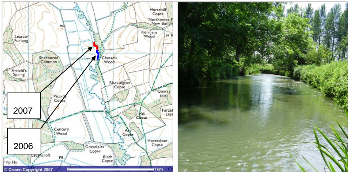
Figure 3:2 Location and typical view of the River Windrush near Sherborne, Gloucestershire. NGR SP 187 156 (Map source: www.ordnancesurvey.co.uk/oswebsite/getmap/ , 25/10/2007.)
