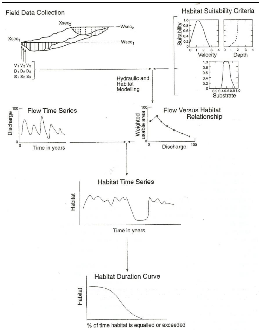
Figure 2:16 The basis of PHABSIM showing the integration of hydraulic measurements and habitat suitability criteria to define the flow/habitat relationship and subsequent combinations with flow time series to produce habitat time series and habitat duration curves (Maddock, 1999, p382).
