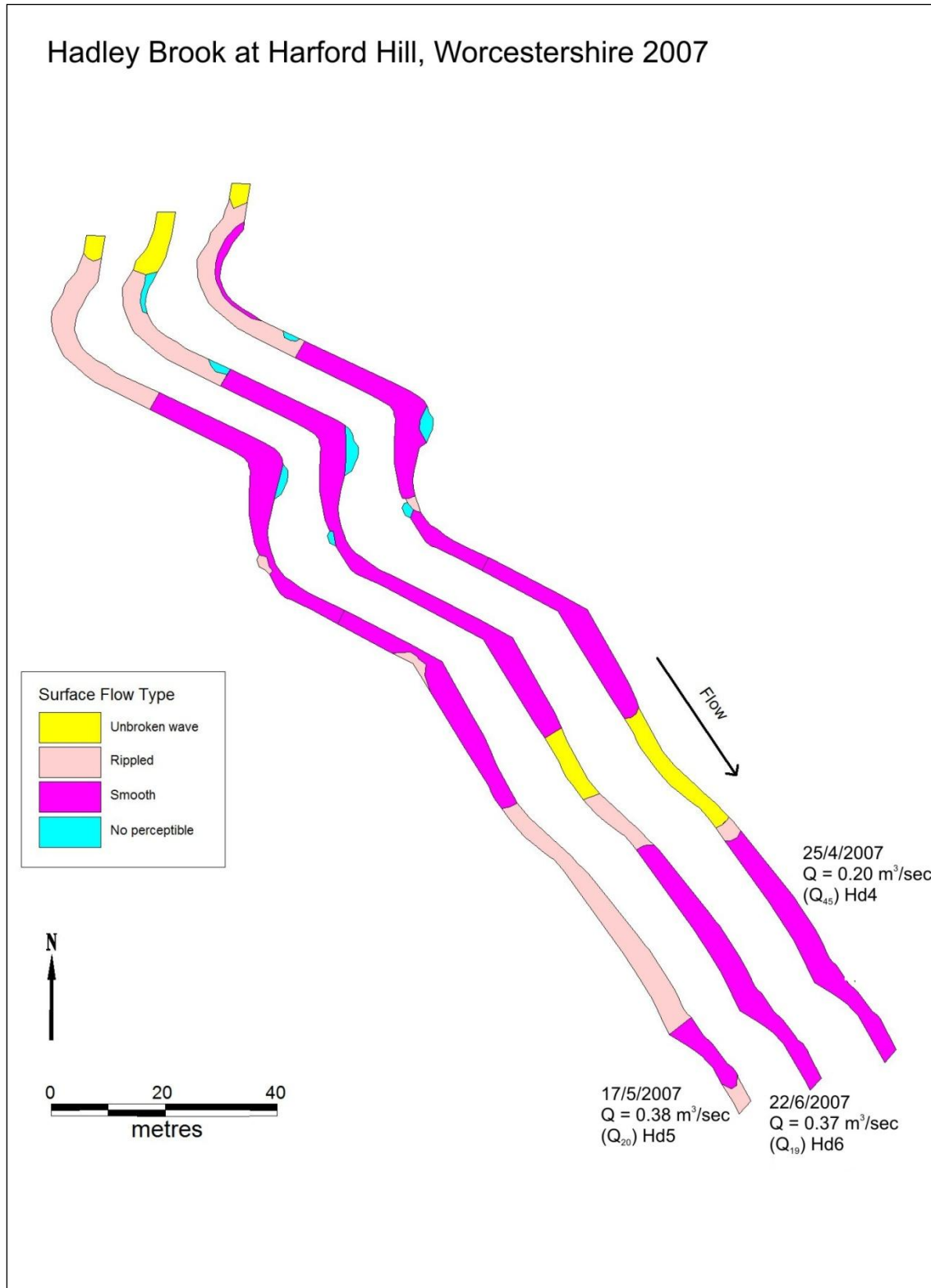
Figure 5:21 Surface Flow Type mesohabitats from three surveys of the same reach of Hadley Brook, Worcestershire in 2007. Key: Hd – Hadley brook, Q – Discharge.
