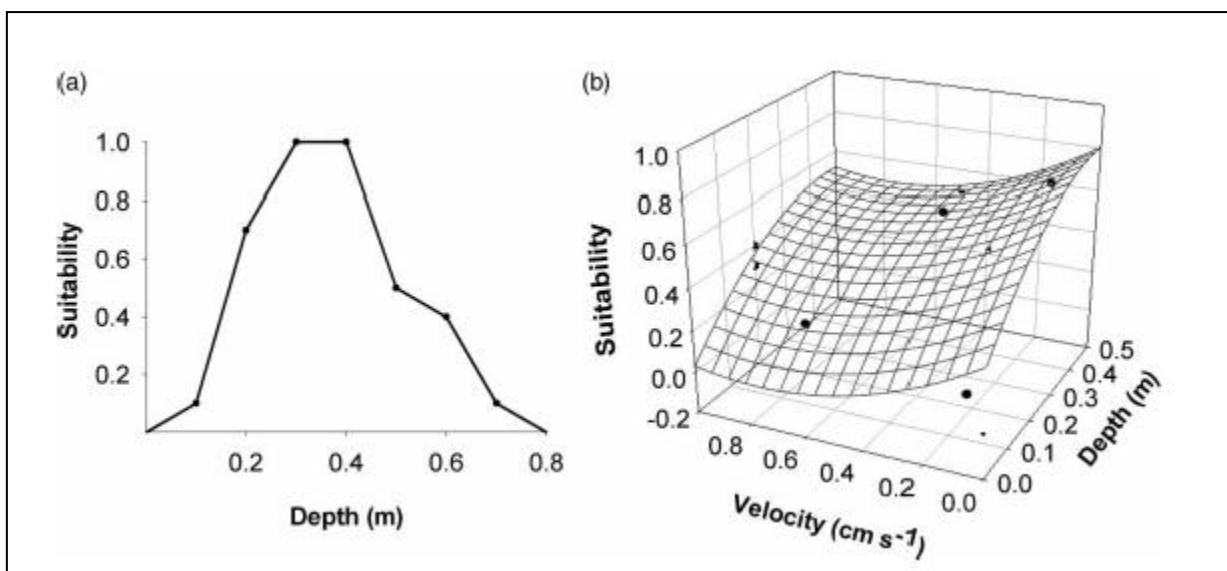
Figure 2:17 Examples showing (a) univariate HSI curve for the habitat variable 'depth' and (b) a multivariate HSI showing the species response to the cumulative effects of both habitat variables depth and velocity (Source: Conallin et al. , 2010, p94).
