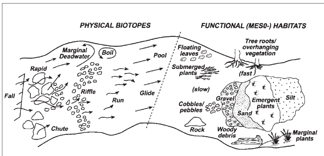
Figure 2:5 A comparison of physical biotopes and functional biotopes. (Newson and Newson 2000, p200).
