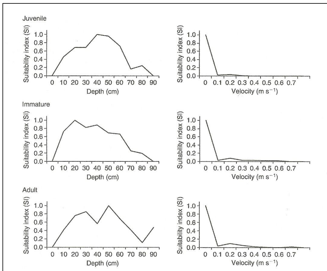
Figure 2:18 Category III Habitat Suitability Curves for two-spined blackfish ( Gadopsis bispinosus ) in the Cotter River (Maddock et al. , 2004, p178)
