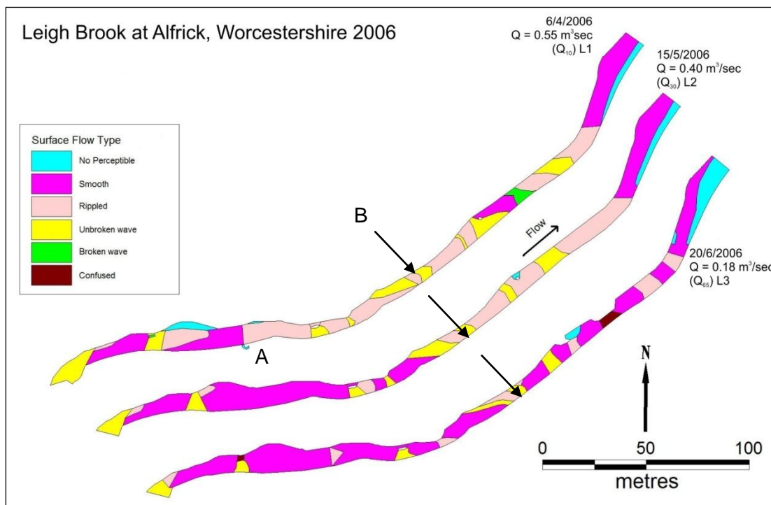
Figure 5:5 Surface Flow Type mesohabitats from three surveys of the same reach of Leigh Brook, Worcestershire in 2006. Key: L – Leigh Brook, Q – Discharge.
